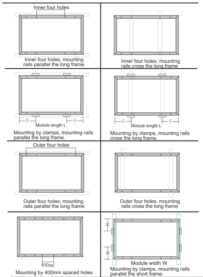
Figure 4 Installation Methods
